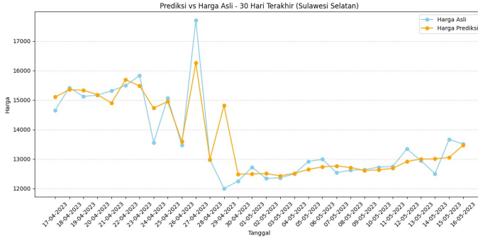
Fig. 2. LSTM: Actual vs. Predicted Rice Prices
