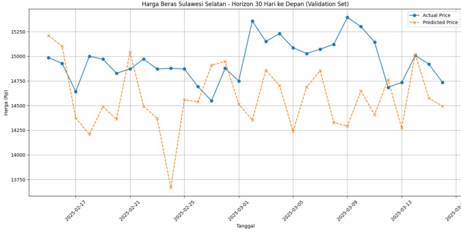
Fig. 3. GNN: Actual vs. Predicted Rice Prices (South Sulawesi, 30-day horizon)
